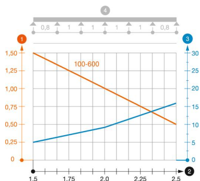
负载图，电缆桥架MKS 60
